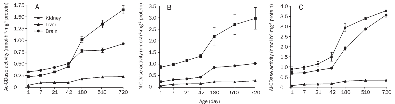
Figure 2. CDase activity in rat kidney, liver and brain tissues. Ac-CDase (A), N-CDase (B) and Al-CDase (C) activities were measured from 7-day, 21-day, 42-day, 180-day, 510-day, and 720-day-old rat kidney, liver and brain tissues. Rat tissue homogenates were incubated with [N-palmitoyl-1- 14 C]-sphingosine. Lipids were extracted and radioactivity of reaction product 14 C-palmitate was counted in a liquid scintillation counter.
